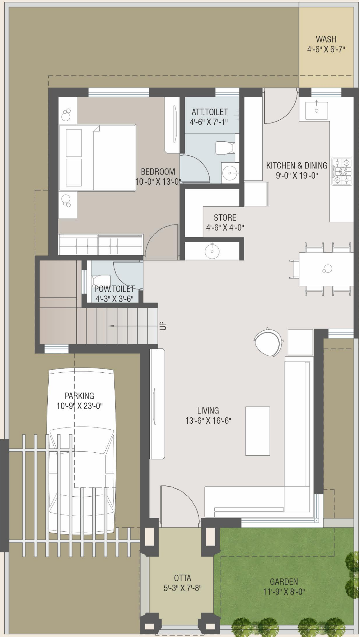
GROUND FLOOR
