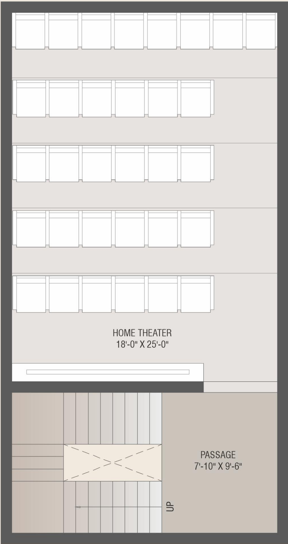
BASEMENT FLOOR
